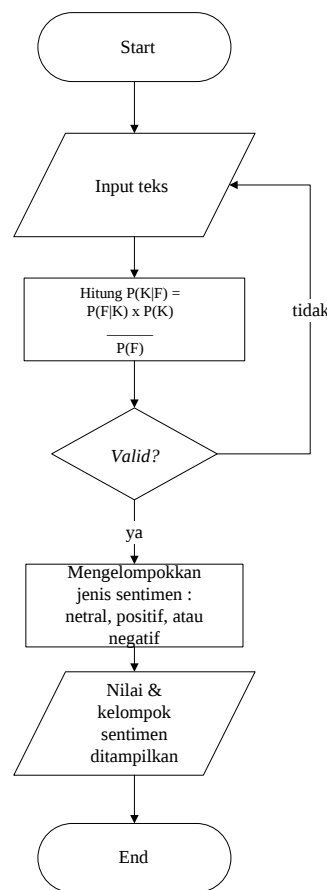
Fig. 1 Naive Bayes Application Calculation Flowchart
