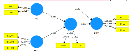
Figure 7. Inner Model Test Results
