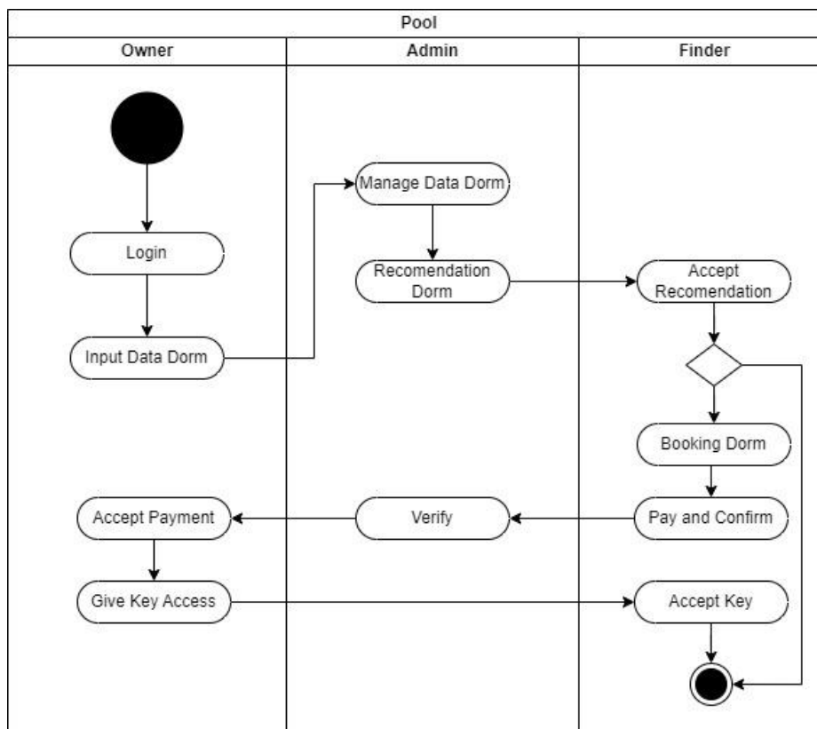
Fig. 2 Activity Diagram
