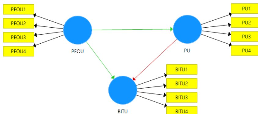
Fig 6 Hypothesis Test Result
