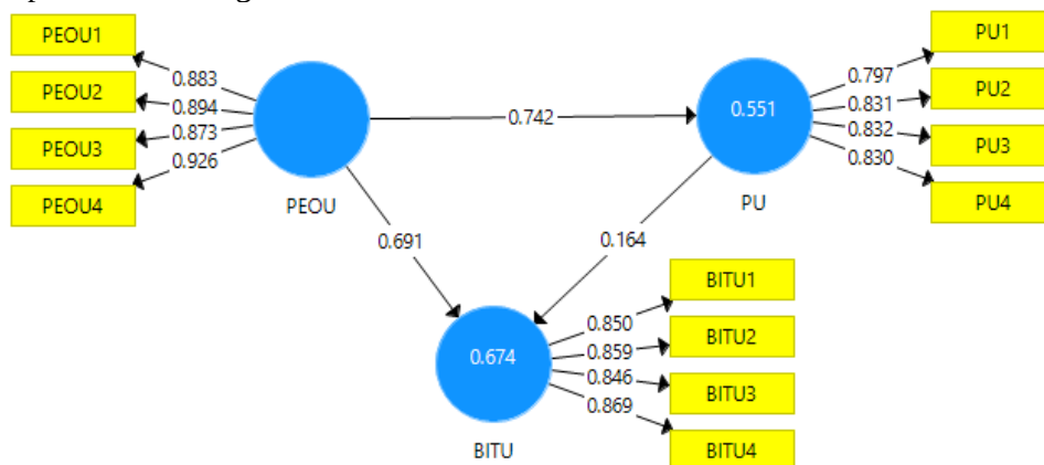
Fig 5 Results of Path Analysis.
