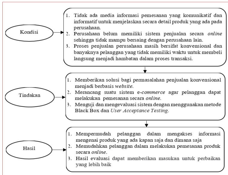
Gambar 1. Diagram Penelitian
