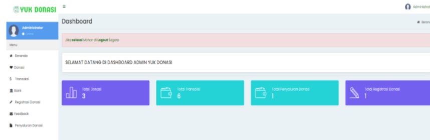
Gambar 2. Halaman Admin
