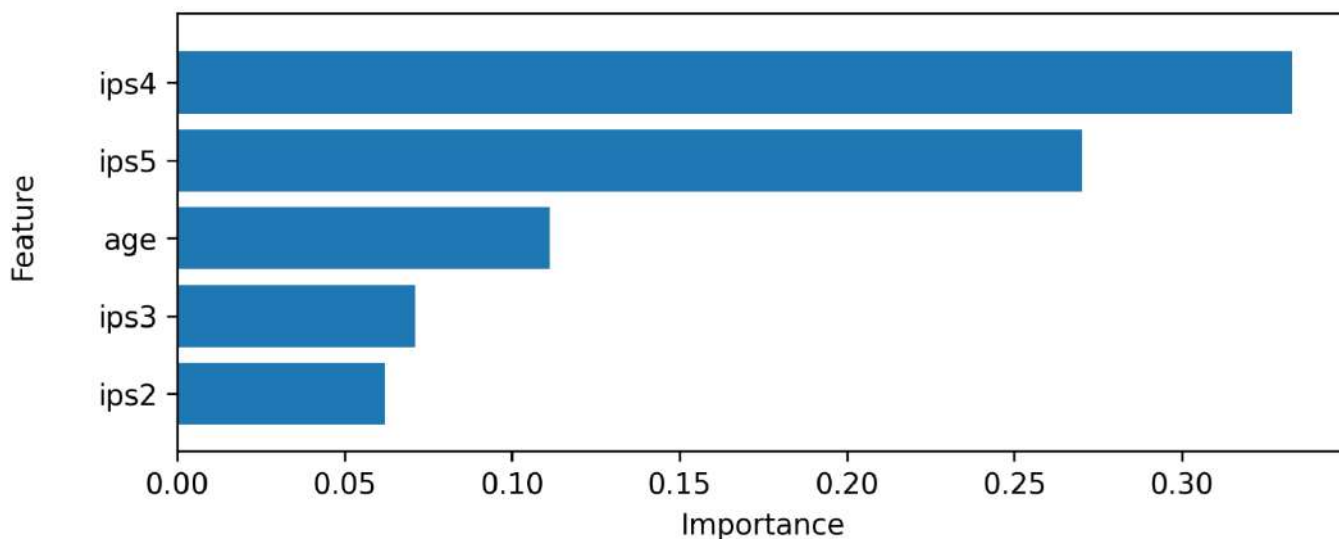
Fig. 4 Top 5 Feature Importance Tuned Random Forest
