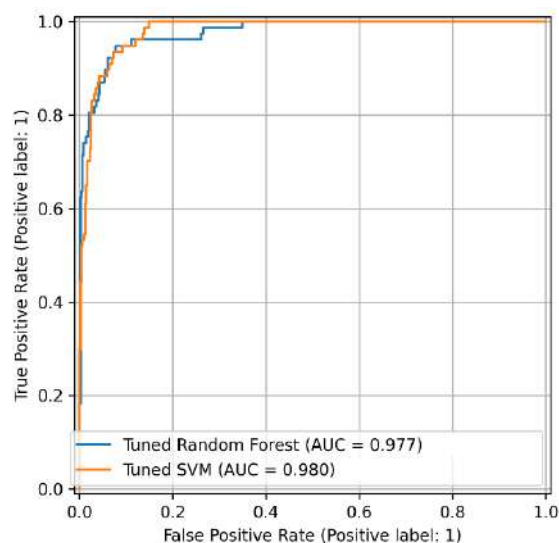
Fig. 3 ROC Curve of Tuned Models
