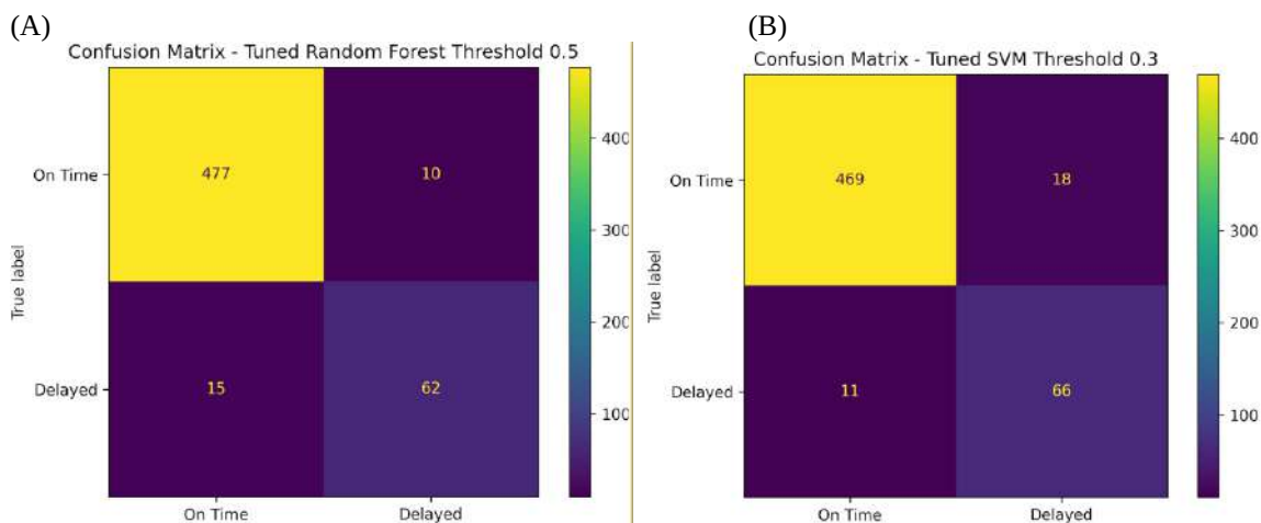
Fig. 2 Confusion matrix (A) Tuned Random Forest, (B) Tuned SVM
