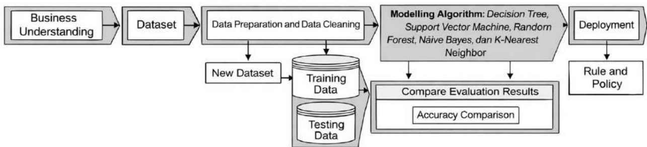
Fig. 1 Proposed Thinking Framework Model
