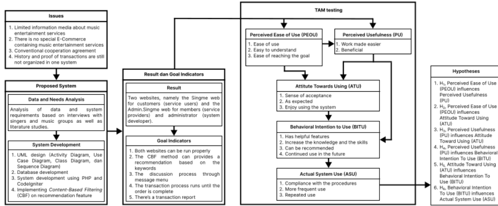
Figure 1. Framework
