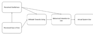
Figure 2. TAM Construct [14]
