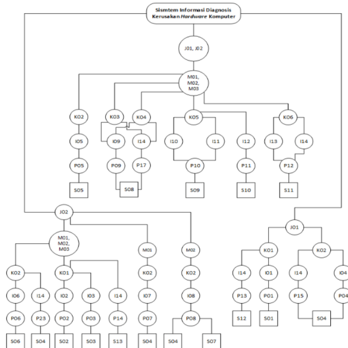
Gambar 4. Rantai Inferensi Diagnosis kerusakan Hardware
