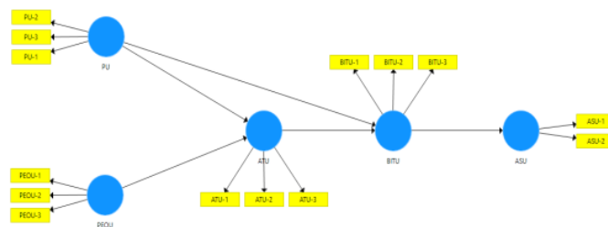
Gambar 7. Path Diagram
