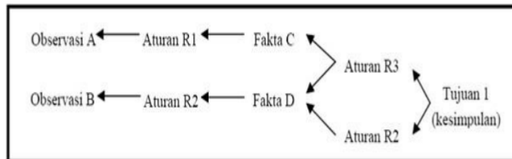
Gambar 2. Proses Backward Chaining
