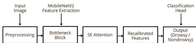
Fig. 1. Research pipeline
