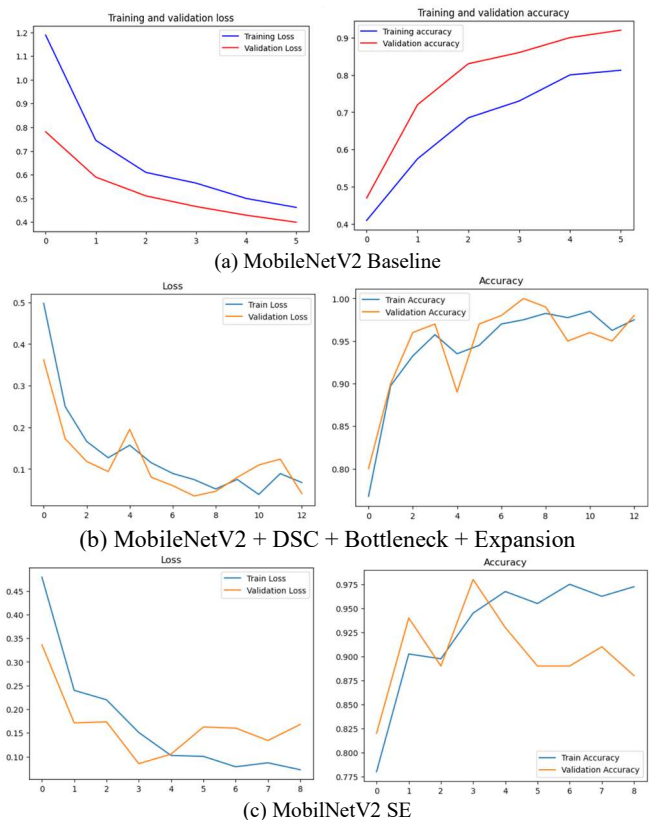
Fig. 3. Training Stability
