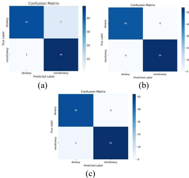
Fig. 4. Confusion Matrix (a) MobileNetV2 Baseline, (b) MobileNetV2 + DSC + Bottleneck + Expansion, (c) MobileNetV2 SE
