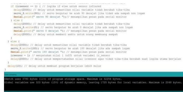
Gambar 7. Perancangan Software (2)
