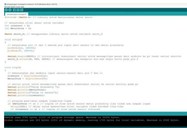
Gambar 6. Perancangan Software (1)
