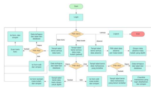
Gambar 4. Flowchart Administrator
