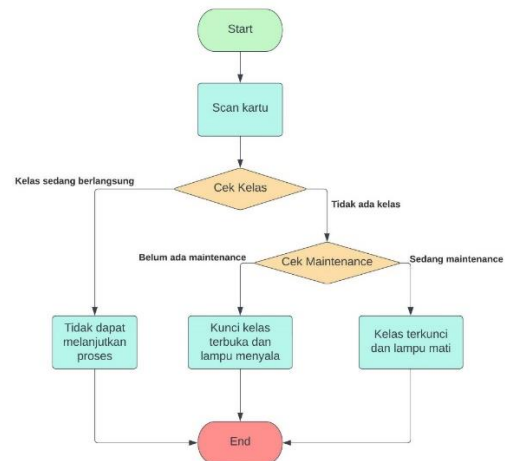
Gambar 3. Flowchart Maintenance
