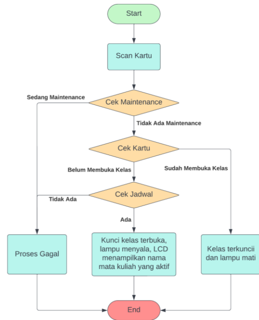
Gambar 2. Flowchart Dosen
