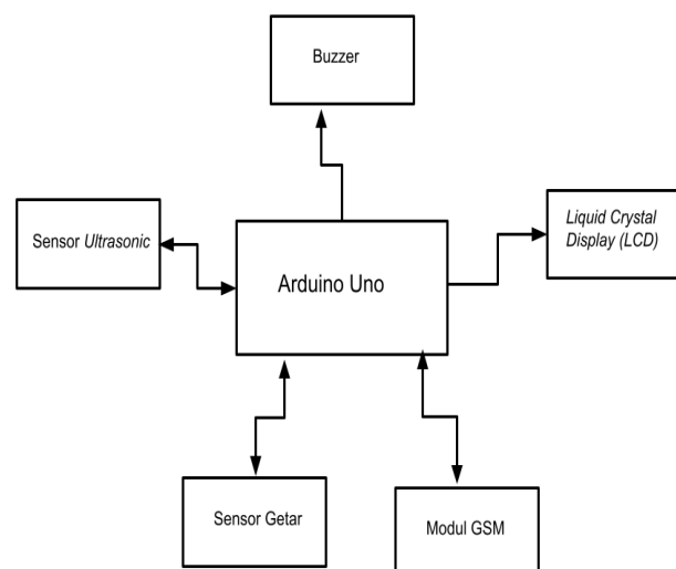
Gambar 2 Block Diagram
