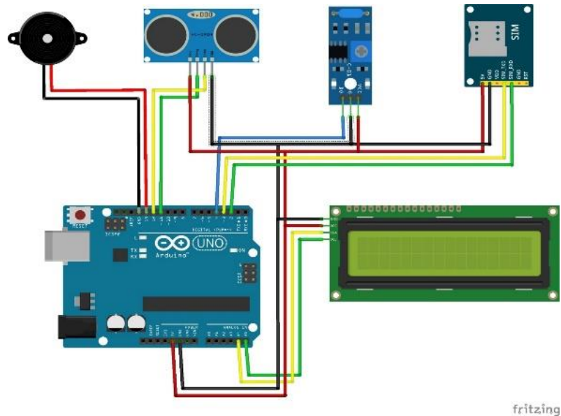
Gambar 3 Wiring Diagram
