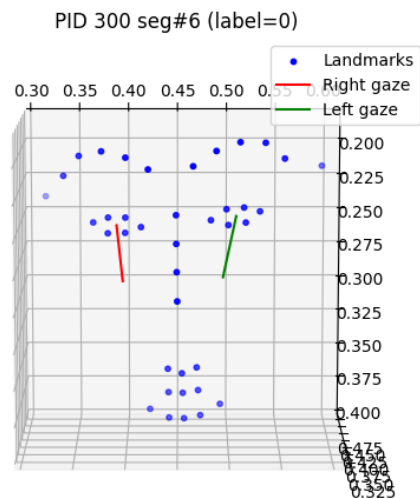
Figure 6 3D visualization of facial landmarks and gaze direction
