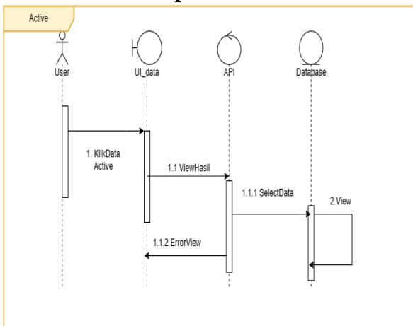
Gambar 12. Sequence diagram active
