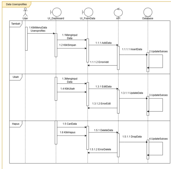
Gambar 11. Sequence diagram data user profiles
