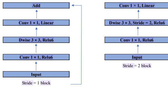
Figure 4. Architectural Structure of MobileNetV2 [25]
