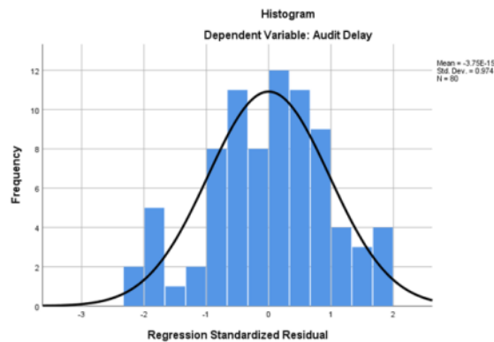
Gambar 2. Hasil Histogram
