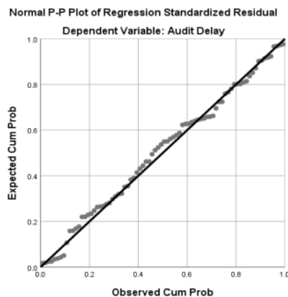
Gambar 3. Hasil Scatterplot
