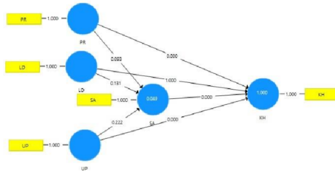
Gambar 1 Hasil Path Analysis
