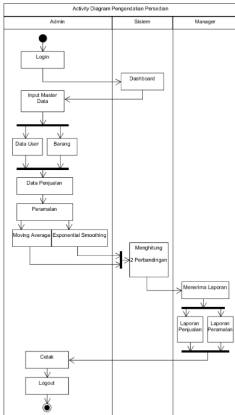
Gambar 1. Activity Diagram
