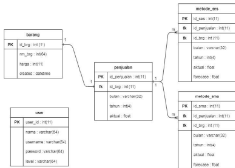
Gambar 2. Class Diagram
