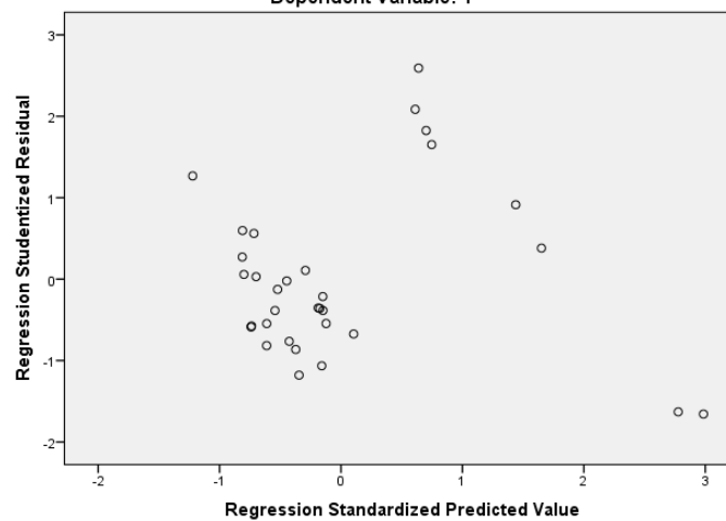
Scatterplot
