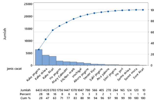
Gambar 3. Diagram pareto
