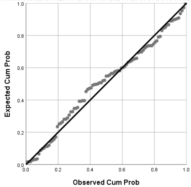
Normal P-P Plot of Regression Standardized Residual Dependent Variable: KEPATUHAN WAJIB PAJAK ORANG PRIBADI
